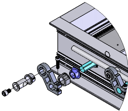
DETAIL B Linkages/Crankarm/Bearings
